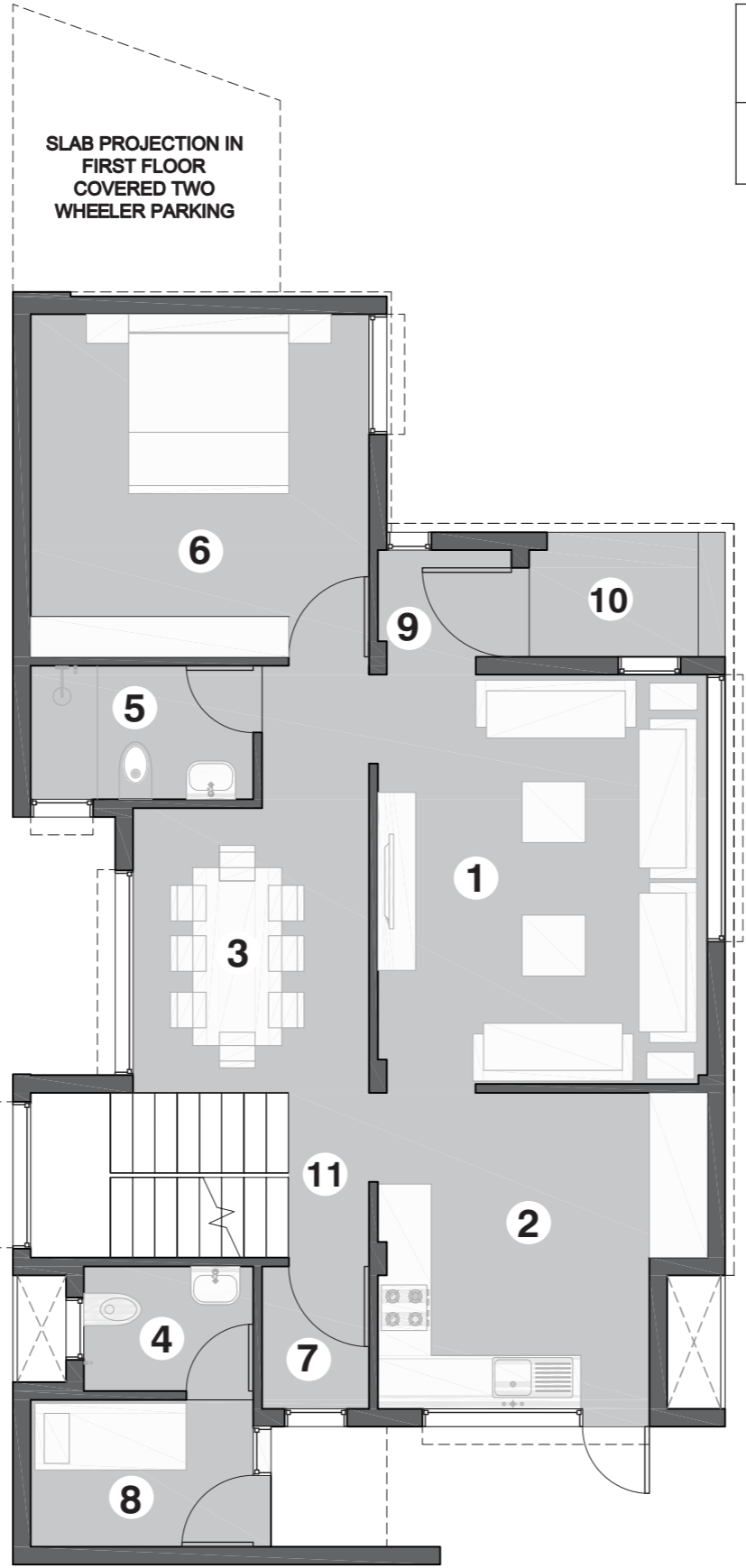
Villa C3-N | GROUND FLOOR PLAN
